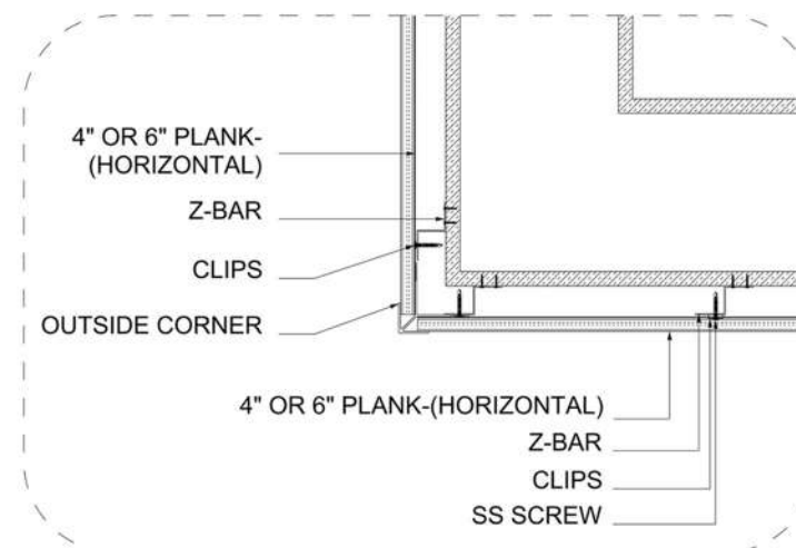
D DETAIL D-12 SCALE: 1.0" 2.0" 5.0"
