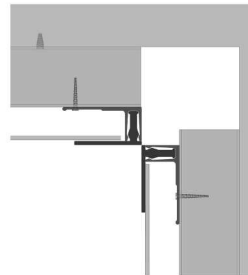
ENLARGED DETAIL B
