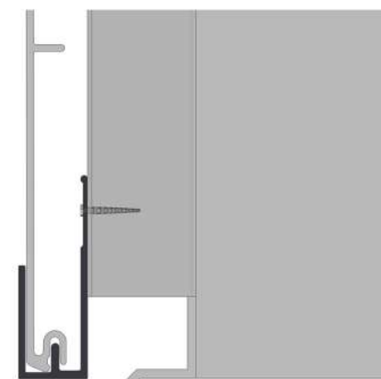
ENLARGED DETAIL C
