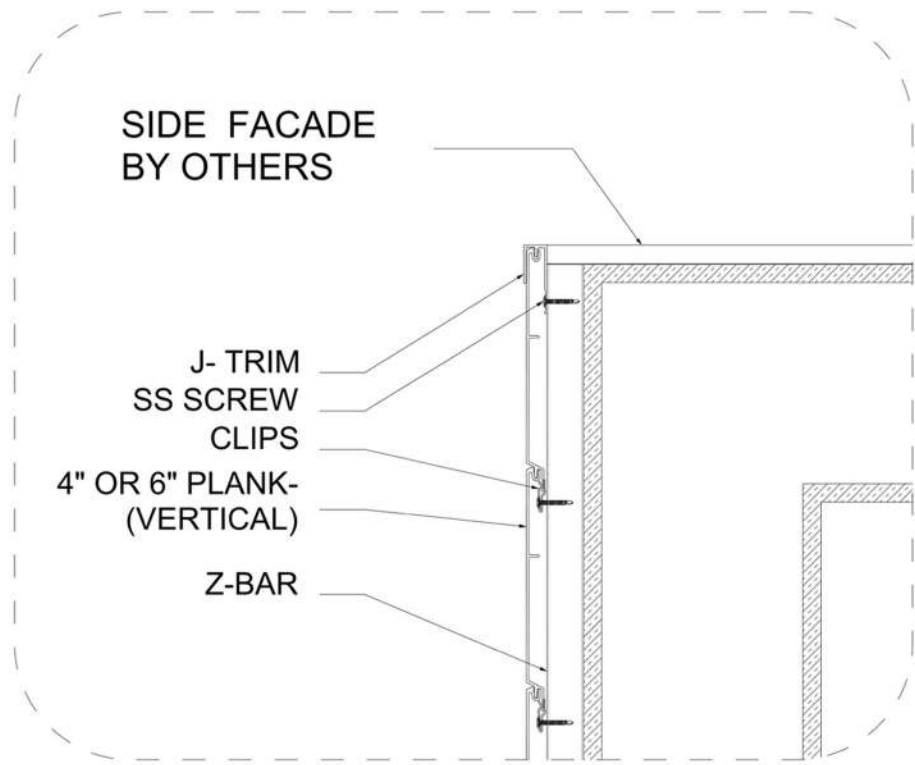
D DETAIL D-01 SCALE: 1.0" 2.0" 5.0"
