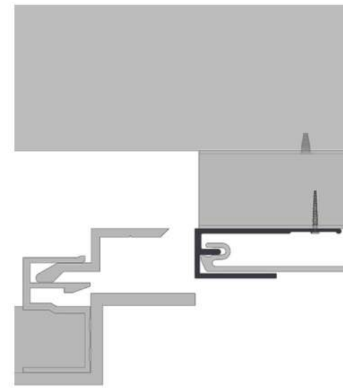
ENLARGED DETAIL A
