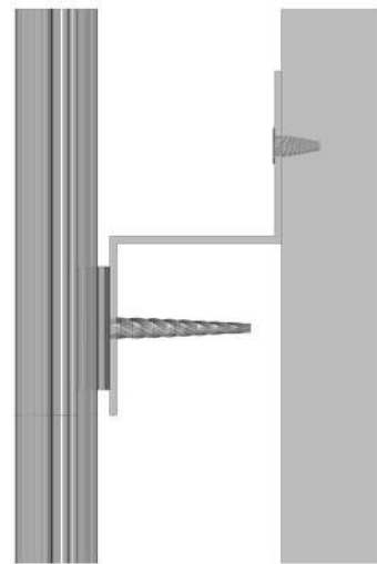
ENLARGED DETAIL B
