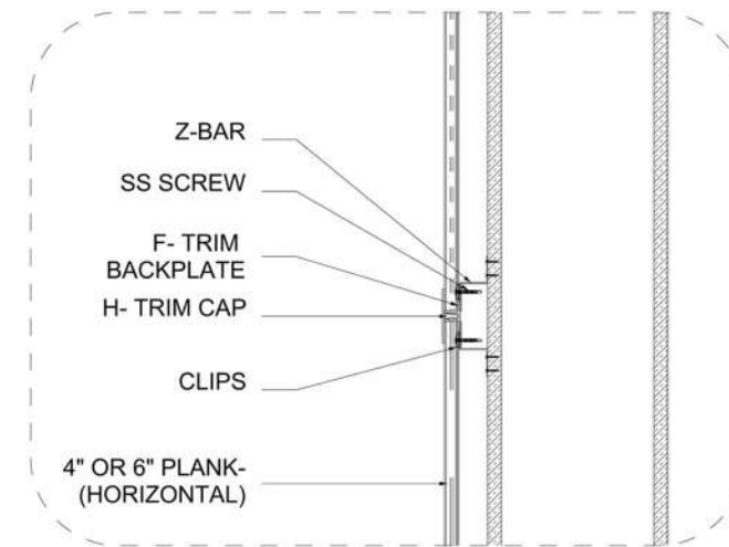
D DETAIL D-11 SCALE: 1.0" 2.0" 5.0"
