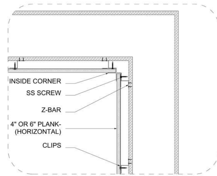
D DETAIL D-10 SCALE: 1.0" 2.0" 5.0"
