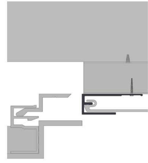
ENLARGED DETAIL A
