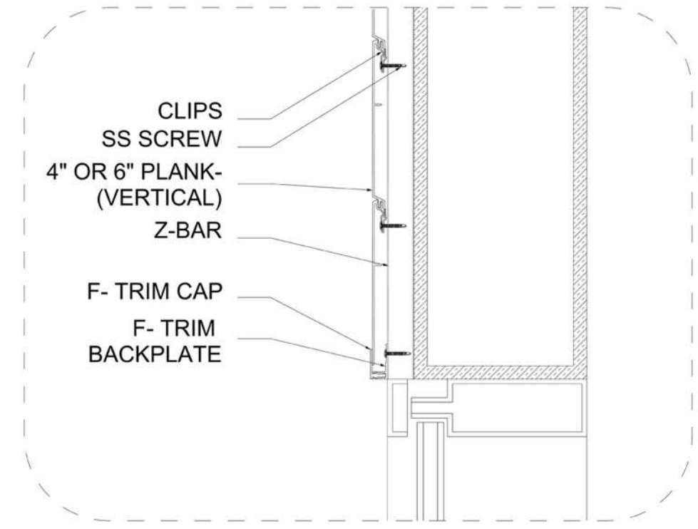
D DETAIL D-02 SCALE: 1.0" 2.0" 5.0"
